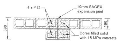
TYPICAL COLUMN SECTION WITH EXPANSION JOINT (EVERY 3rd COLUMN) SCALE 1:20
