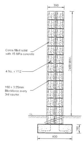
TYPICAL SECTION THROUGH COLUMN SCALE 1:25
