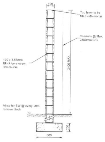
TYPICAL SECTION THROUGH WALL SCALE 1:25
