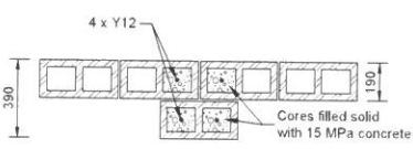
TYPICAL COLUMN SECTION WITHOUT EXPANSION JOINT SCALE 1:20
