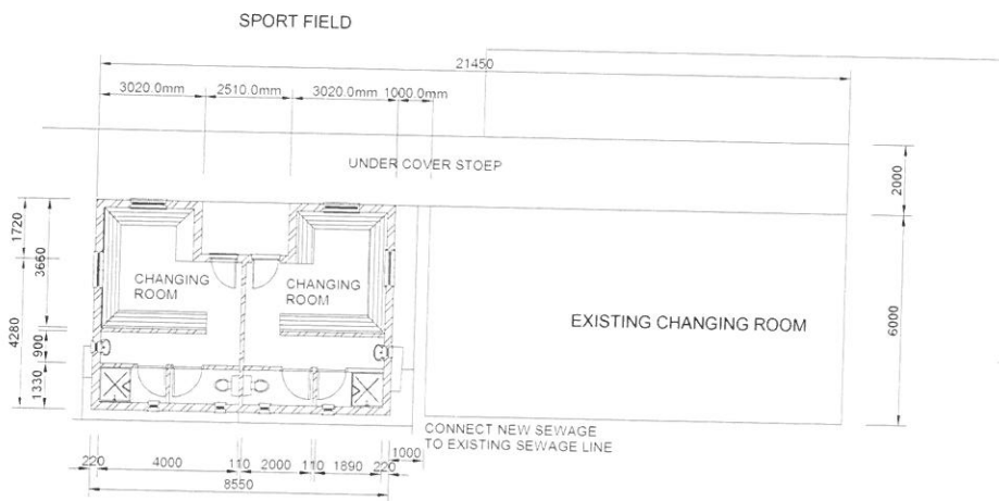
FLOOR PLAN KLAARSTROOM SPORT FIELD SCALE 1:100
