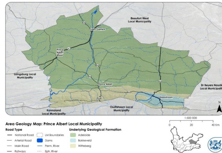
Figure 3.2: Area Geology Map of PAM
