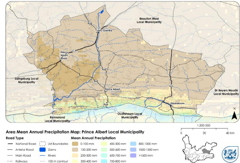
Figure 3.8: Annual Precipitation of PAM
