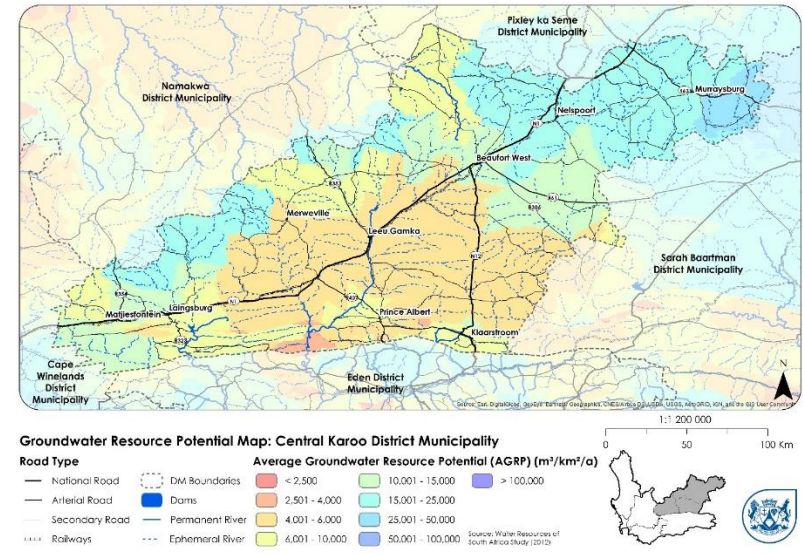
Figure 3.9: Groundwater Resources Potential Map for CKDM
