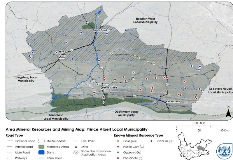
Figure 3.3: Area Mineral Resources Map of PAM
