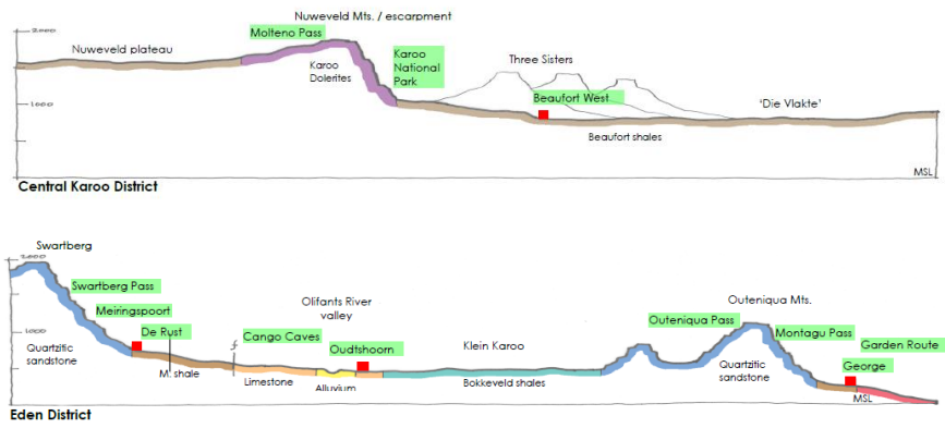
Figure 3.6: Landscape Typology Cross section of Central Karoo and Eden Districts
