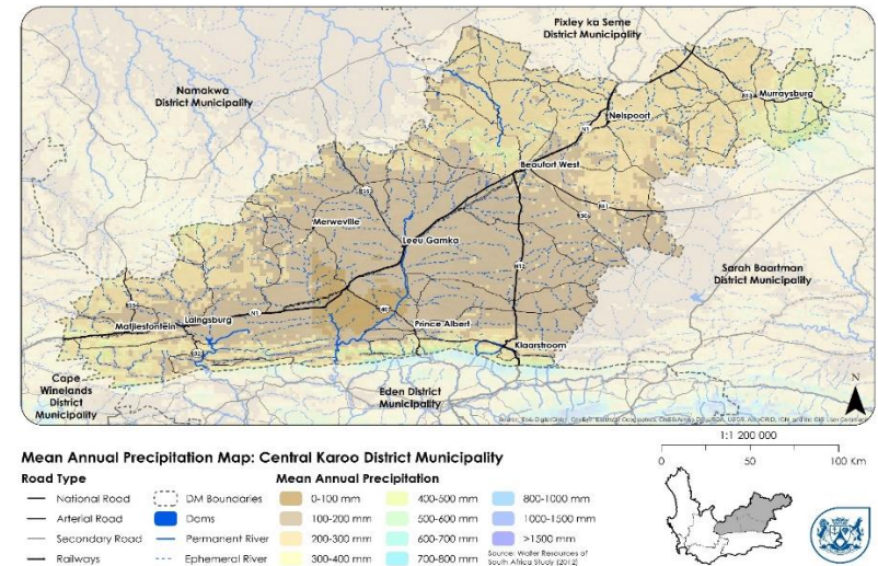
Figure 3.7: Annual Precipitation of CKDM
