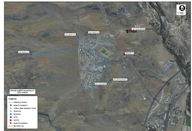
Figure 3.40: Water Infrastructure in Bitterwater
