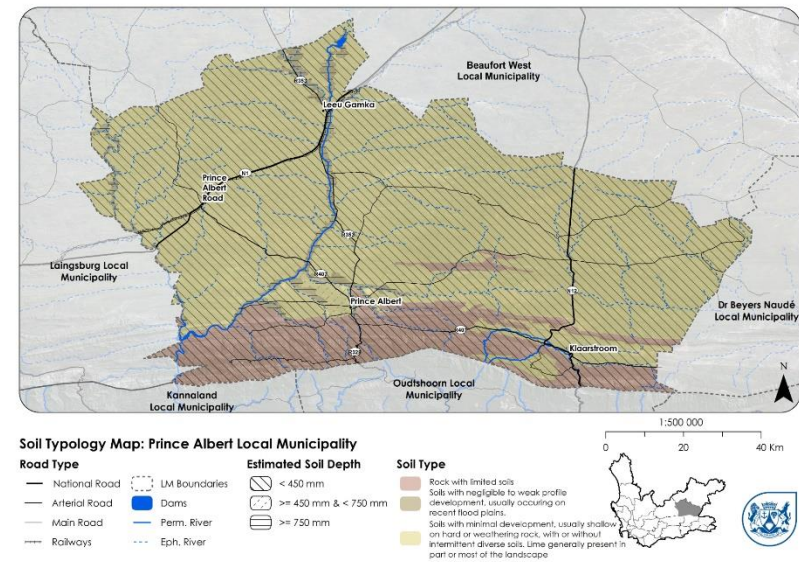
Figure 3.4: Soil Typology Map of PAM
