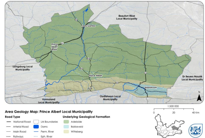
Figure 3.5: Geology Map of PAM
