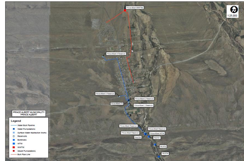
Figure 3.39: Water Infrastructure in Prince Albert Town
