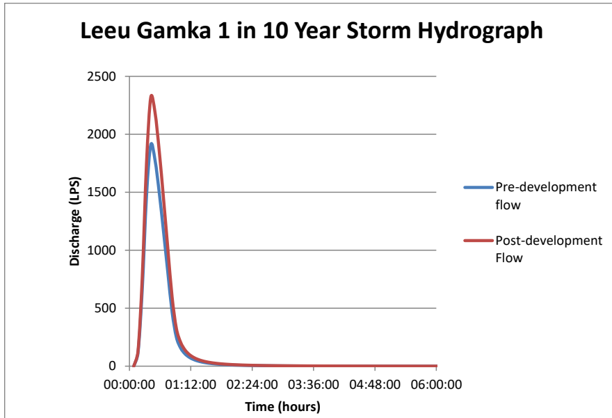
Figure 7.3: Leeu Gamka 1 in 10 Year Storm Hydrograph
