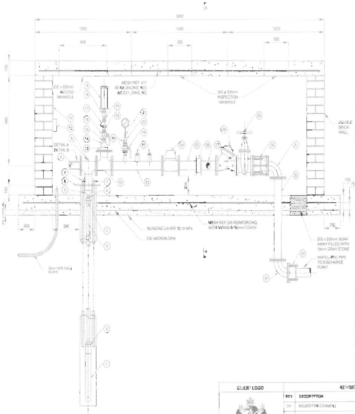
SECTION B-B
